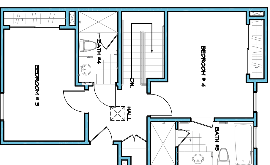
UNIT E THIRD FLOOR PLAN
