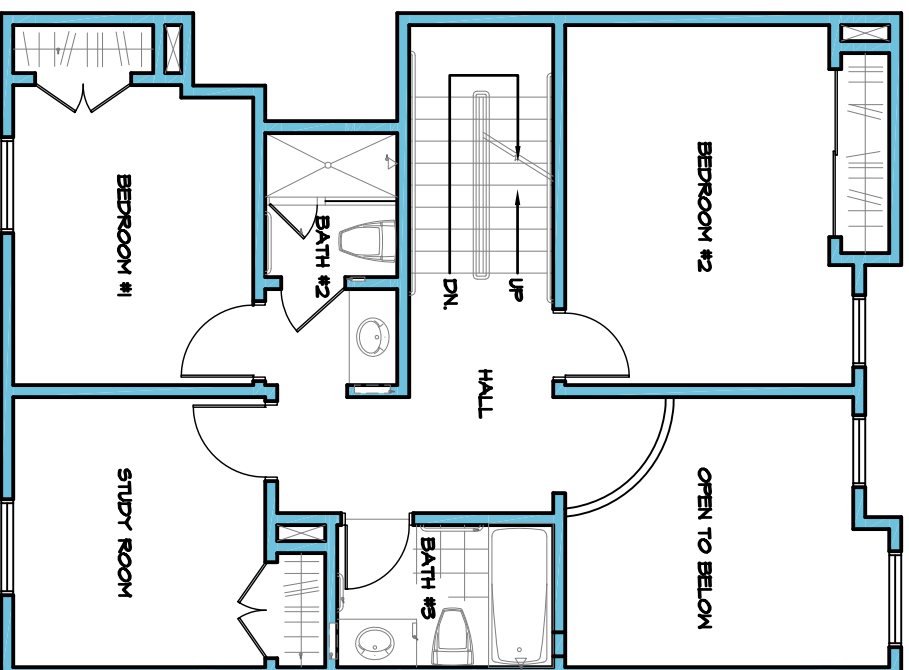
UNIT A-2 SECOND FLOOR PLAN
