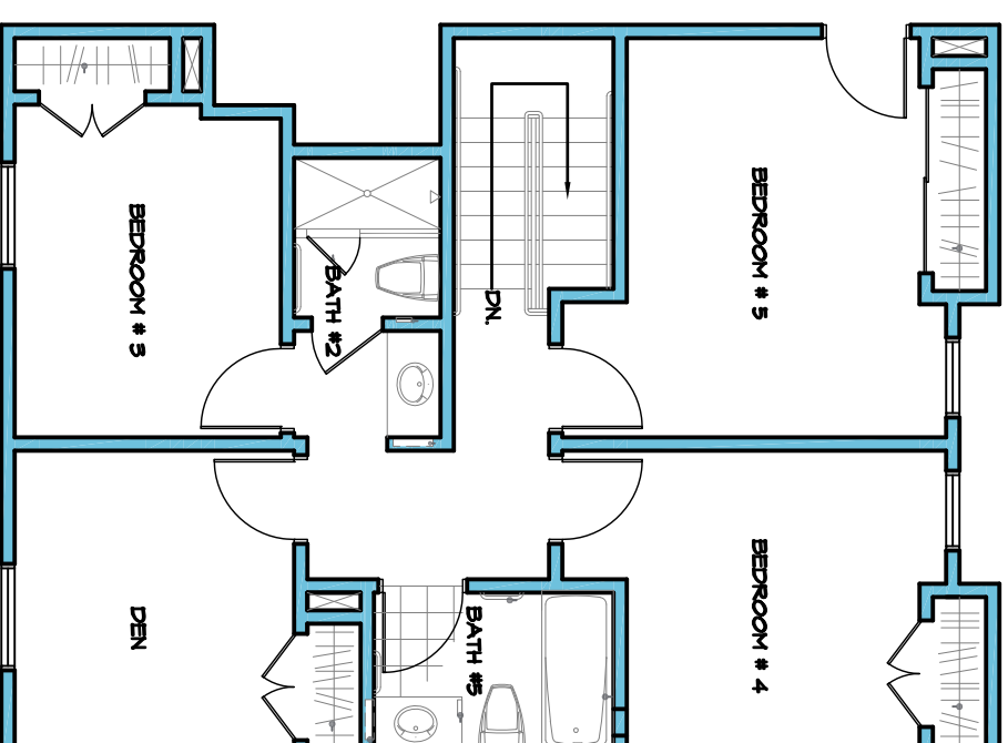
UNIT A-2 THIRD FLOOR PLAN
