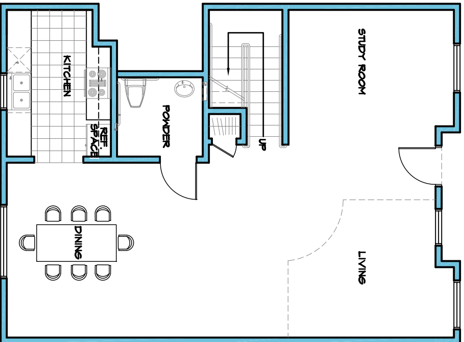
UNIT A-2 FIRST FLOOR PLAN
